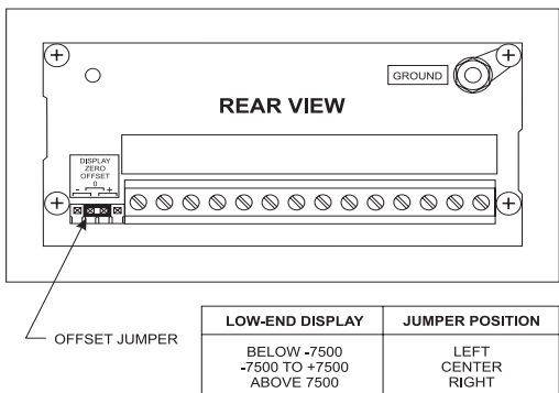
Figure 3 Display Zero Offset Jumper (4½ Digit Only)
